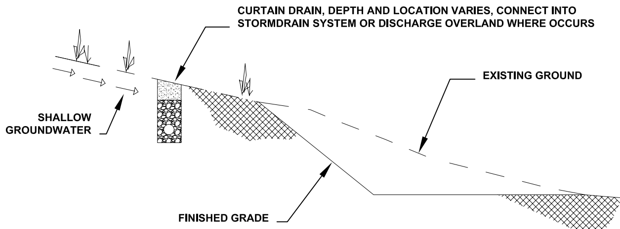
5-9A. CUT SECTION
