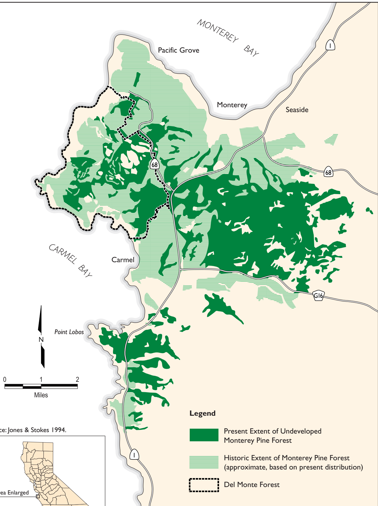
Figure E-2 Distribution of Native Monterey Pine Forest in the Monterey Region
