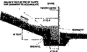
1. RECOMMENDED INSTALLATION OF SILT FENCE
