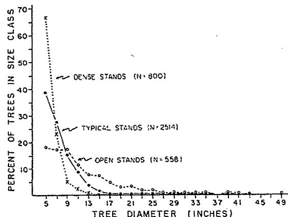
Percentage distribution of size classes in three categories of foothill woodland. Over 90% of the trees sampled were less than 12 inches dbh.
