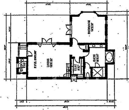
CARETAKER FLOOR PLAN SCALE: 1/8" = 1'-0"
