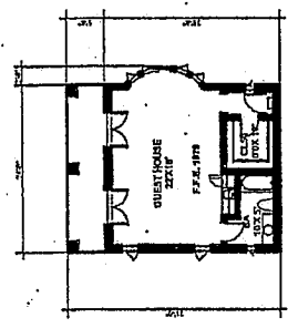
GUEST HOUSE FLOOR PLAN SCALE: 1/8" = 1'-0"
